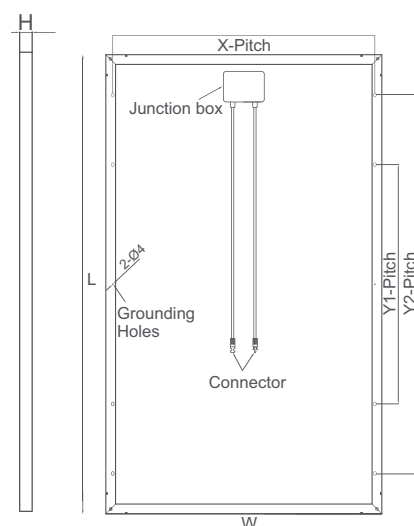
Module & Mounting Dimensions
